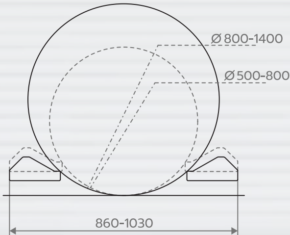
ROLL DIAMETER
